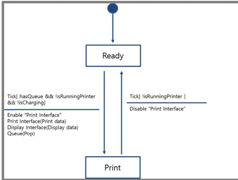
3.2.5.4.3 STD for Controller 2.1.3.1
